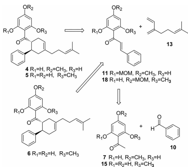
Scheme 1. Retrosynthetic analysis of natural products 4-6 .
