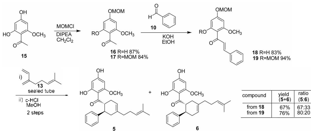
Scheme 3
