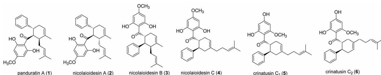
Figure 1. Selected naturally occurring dihydrochalcones.
