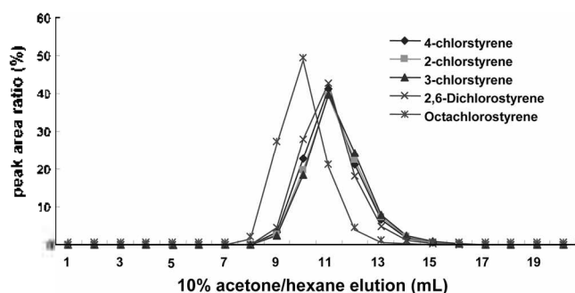
Figure 3. Elution patterns of chlorostyrenes on Florisil-SPE cartridge with acetone/ n -hexane (1:9, v/v).
