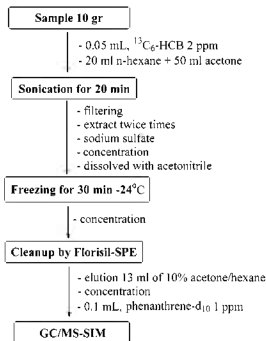
Figure 2. Analytical procedure of chlorostyrenes for fish tissue sample.
