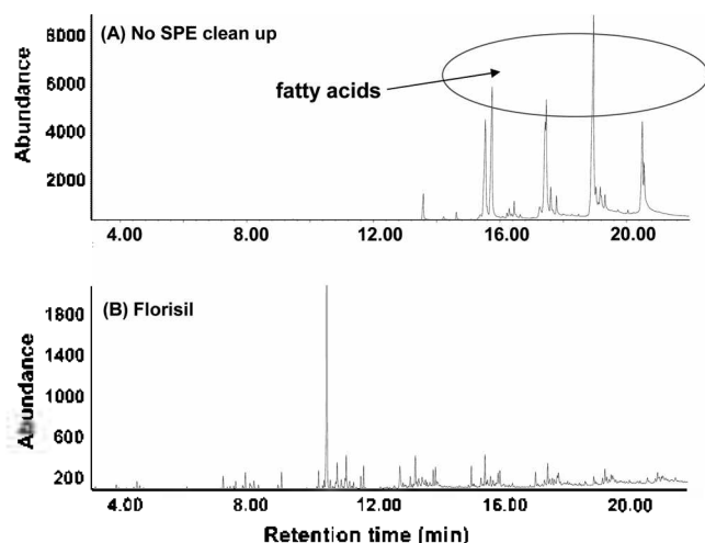
Figure 4. Total ion chromatograms of blank fish extracts after freezing-lipid filtration: no clean up (A) and Florisil-SPE (B).
