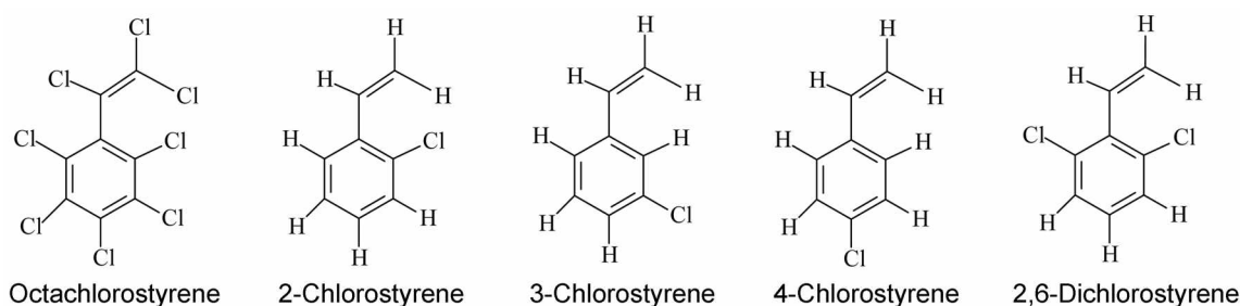
Figure 1. Chemical structures of chlorostyrenes investigated in this study.
