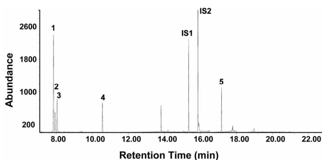
Figure 5. GC-MS-SIM chromatogram of chlorostyrenes in spiked fish sample at 10 ppb. Peak identities: 1, 4-chlorostyrene, 2, 2-chlorostyrene, 3, 3-chlorostyrene, 4, 2,6-dichlorostyrene, 5, octachlorostyrene, phenanthracene- d_{10} (IS1) and ^{13}\text{C}_6 -HCB (IS2).
