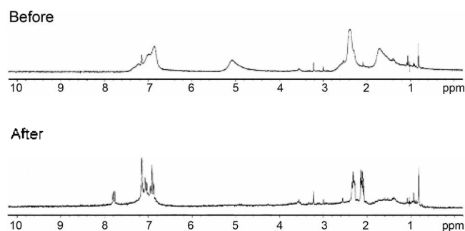
Figure 1. ^1\text{H} NMR spectra before and after irradiation of PMPMA in benzene d_6 .
