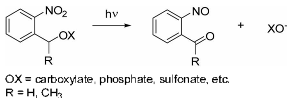
Scheme 1. Photochemical reaction of o -nitrobenzyl esters.
