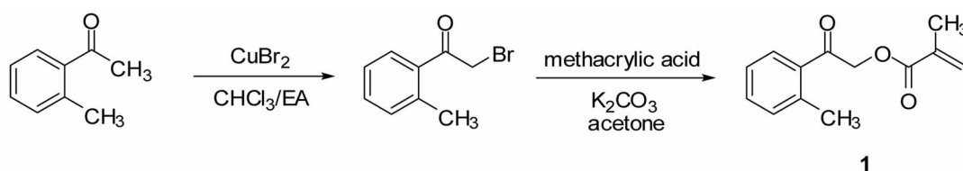
Scheme 2. Synthesis of the Monomer.
