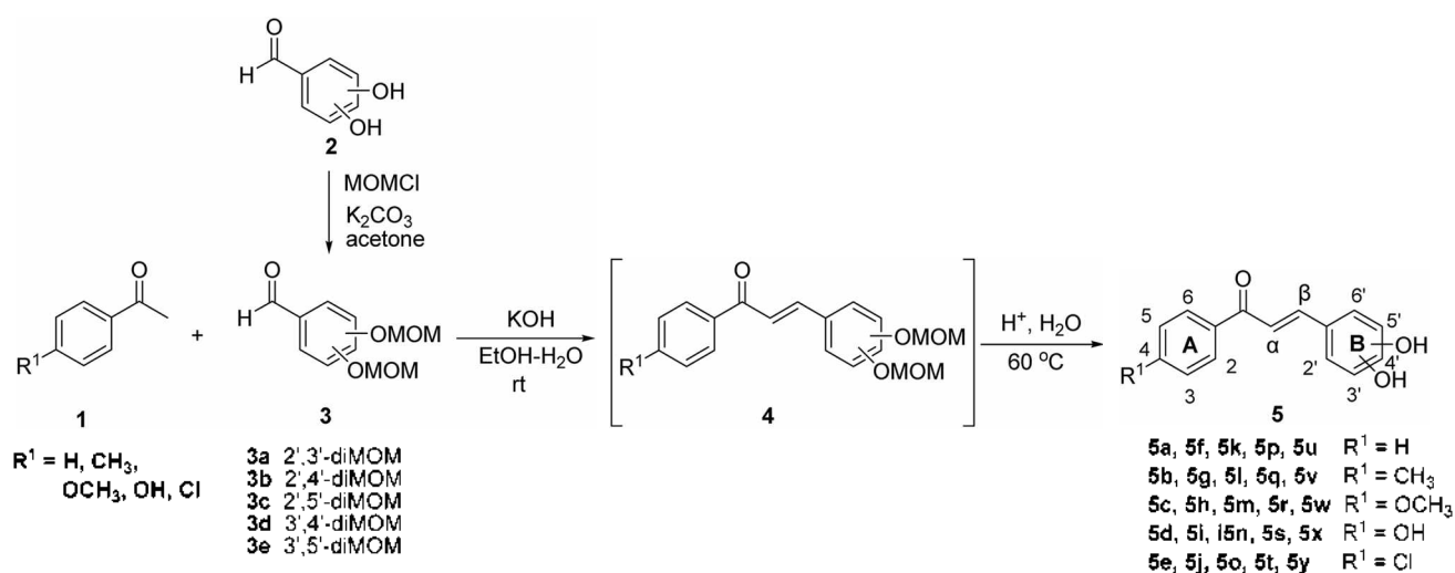
Scheme 1. General procedure for the formation of chalcones 5 .
