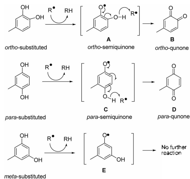
Figure 2. Proposed rationale for strong activity of ortho - and para -dihydroxylated chalcones vs meta -dihydroxylated ones.
