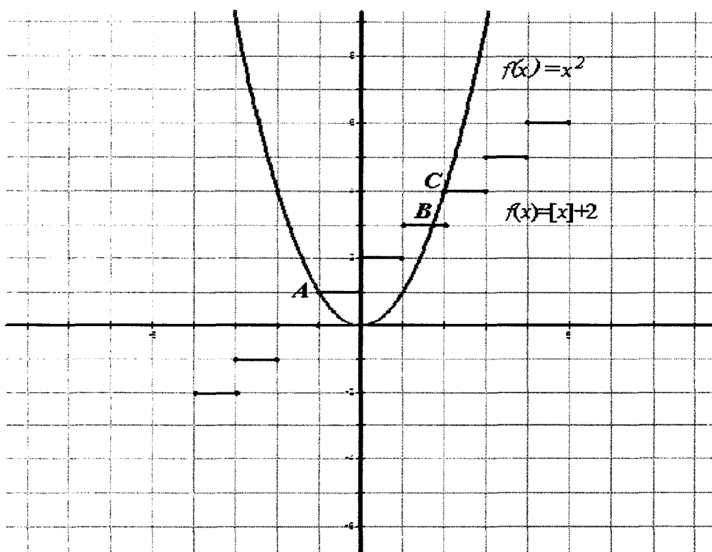
Figure 1. Graphical solution method
