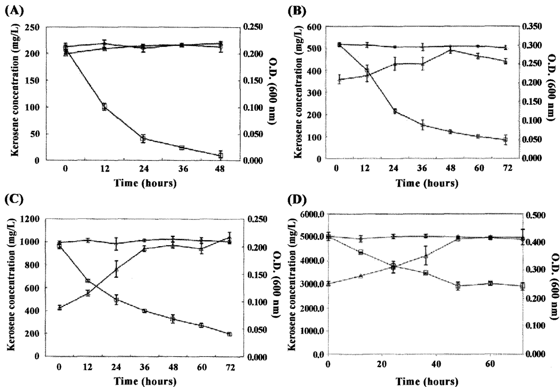
Fig. 1. Biodegradation of Kerosene by Pseudomonas aeruginosa K14 strain. Cell concentration: 1.0 g/L (w/v), temperature: 30°C. pH 7, initial substrate concentration: (A) 200 mg/L, (B) 500 mg/L, (C) 1,000 mg/L, (D) 5,000 mg/L (◇) control, (□) biodegradation, (△) cell growth.
