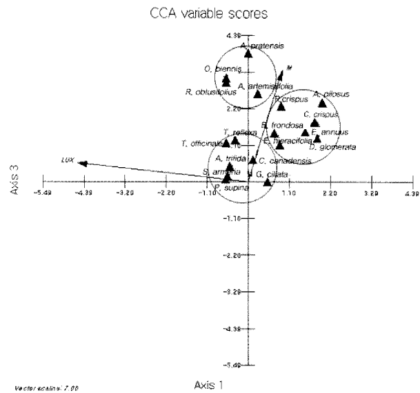
Fig. 5. Result of CCA (canonical correspondence analysis) for the illuminance and distance into the forest.
