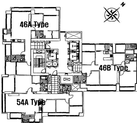
Fig. 1 102 Block floor plan.
