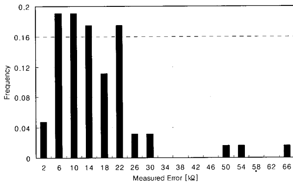
Fig. 6. Measured errors between proposed relative measurement methods and external impedance meters. The mean and standard deviation of the measured errors are 13.9 k \Omega , and 11.7 k \Omega , respectively.
