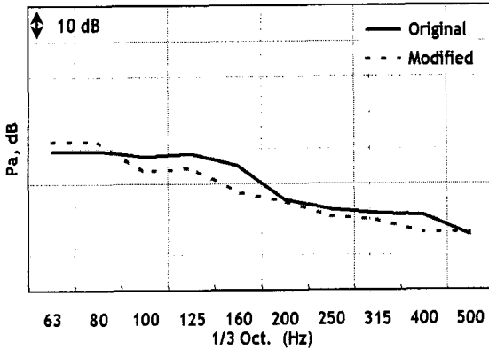
Fig. 12 Sensitivity test result through test by modifying NTFs and accelerations for BODY 1, 2 and 5
