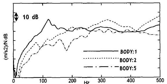
(b) Vibration transfer function (accelerance)
