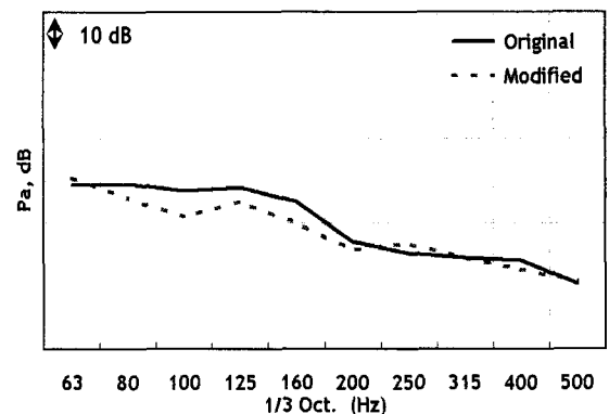
Fig. 11 Sensitivity test result through test by decoupling 3 points : BODY 1, 2 and 5
