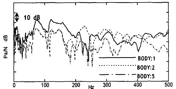
(a) Noise transfer function
