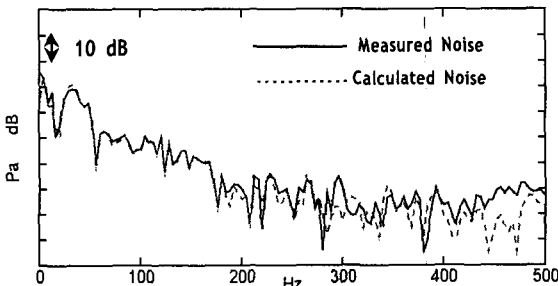
Fig. 5 Comparison of measured and calculated noise
