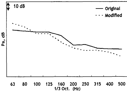
Fig. 10 Sensitivity analysis result through TPA model by modifying NTFs and accelerations for BODY 1, 2 and 5
