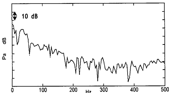
Fig. 3 Frequency spectrum of 1st slosh noise
