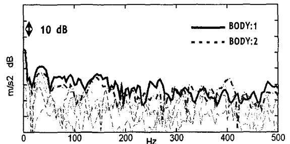
Fig. 7 Accelerations applied at body attachment point
