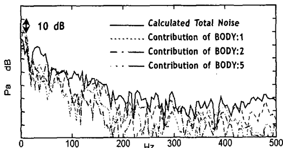
Fig. 6 Contribution of connection points to interior noise
