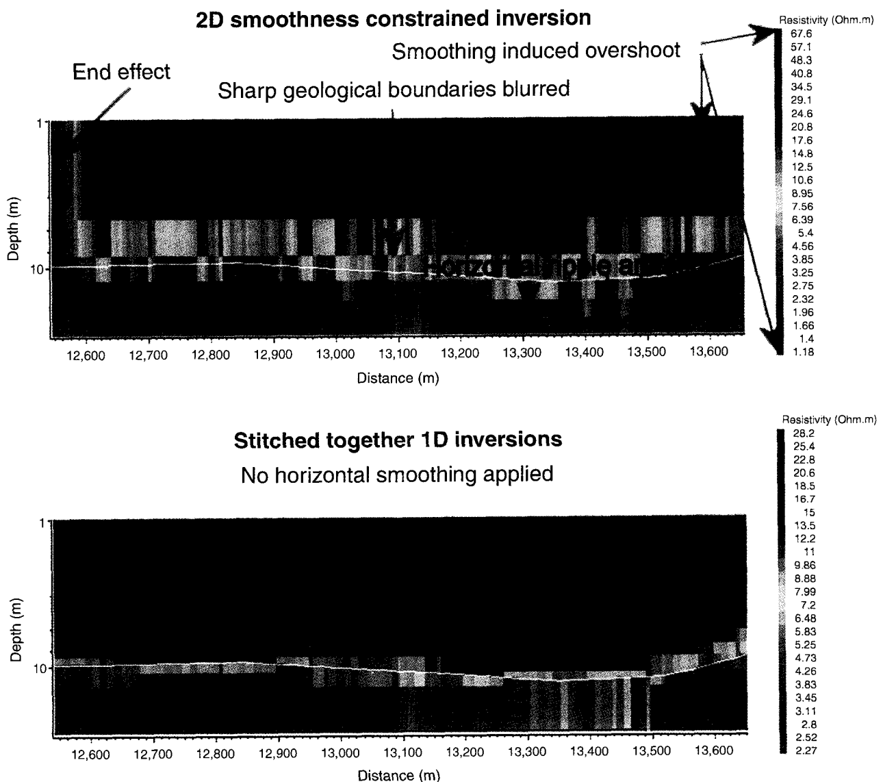
Fig. 1. A comparison of 2D and 1D inversion of one 1 km long segment of riverborne geo-electric data collected with a dipole-dipole array. An aqua line represents the approximate depth of the river bed. 1D inversion works more effectively with an array with an exponential distribution of receiver electrodes but 2D inversion of data collected with such an array is not very practical. For comparison purposes, 1D inverted data has not been horizontally smoothed as would normally be done to reduce the effect of noise.
