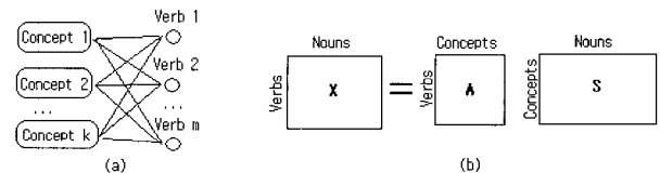
Fig. 2. The illustration of the ICA model from concept views: a) verbs act like microphones, indicating the mixture of concepts via their noun usage. b) The model in matrix notation.
