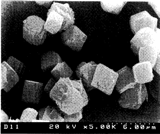
Figure 6. Scanning electron micrograph of ETAS-10 sample.
