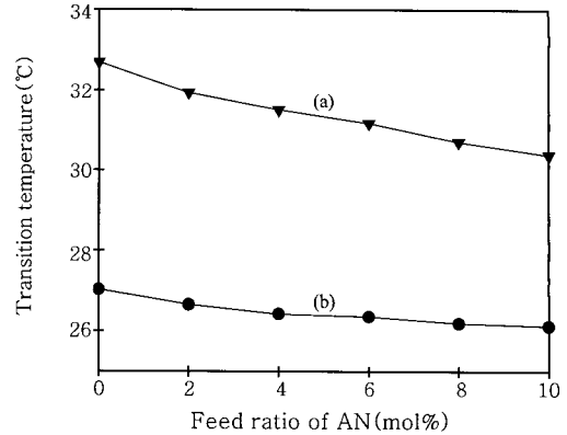
Figure 12. Effect of feed ratio of AN on the CGTT of P(NIPAAm-co-AN) hydrogels determined from the DSC curves of (a) heating and (b) cooling process.
