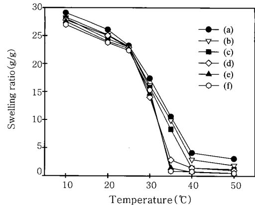
Figure 5. Temperature dependence of the swelling ratio of P(NIPAAm-co-AN) hydrogels. Feed ratio of AN (mol %); (a) 0 (PNIPAAm), (b) 2, (c) 4, (d) 6, (e) 8, and (f) 10.
