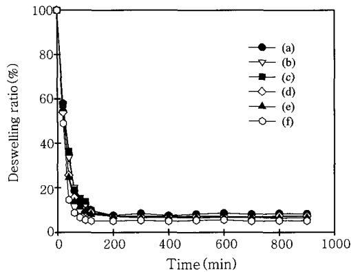
Figure 7. Deswelling ratio of P(NIPAAm- co -AN) hydrogels at 50 °C as a function of time. Feed ratio of AN (mol%); (a) 0 (PNIPAAm), (b) 2, (c) 4, (d) 6, (e) 8, and (f) 10.
