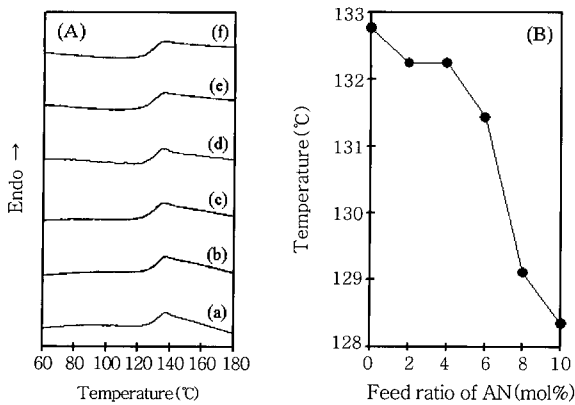
Figure 4. (A) DSC heating thermograms of P(NIPAAm-co-AN)s with various feed ratios of AN (mol %); (a) 0 (PNIPAAm), (b) 2, (c) 4, (d) 6, (e) 8, and (f) 10. (B) Change in T_g of P(NIPAAm-co-AN) copolymer with feed ratio of AN.
