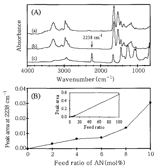
Figure 1. (A) Normalized FTIR-ATR spectra of (a) PNIPAAm, (b) P(NIPAAm- co -AN) with 10 mol% of AN, and (c) PAN. (B) Effect of AN content on the peak area at 2238 \text{cm}^{-1} for P(NIPAAm- co -AN).
