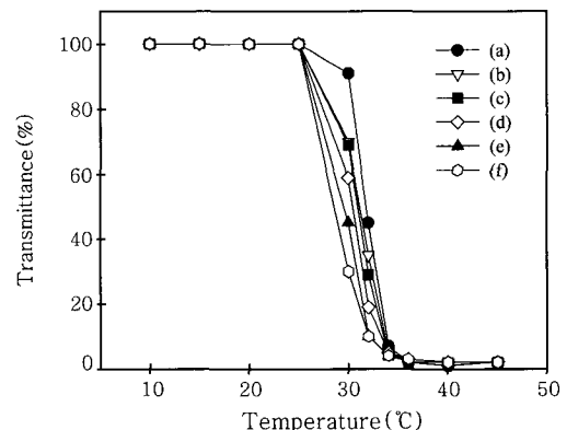
Figure 2. Sharp decrease in transmittance of the aqueous solution of P(NIPAAm- co -AN) with increasing temperature. Feed ratio of AN (mol%); (a) 0 (PNIPAAm), (b) 2, (c) 4, (d) 6, (e) 8, and (f) 10.
