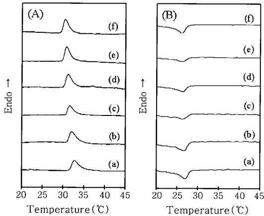
Figure 11. (A) Heating and (B) cooling DSC thermograms of P(NIPAAm-co-AN) hydrogels. Feed ratio of AN (mol%); (a) 0 (PNIPAAm), (b) 2, (c) 4, (d) 6, (e) 8, and (f) 10.
