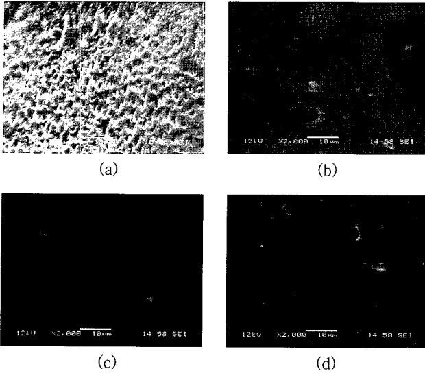
Figure 10. SEM images of freeze-dried P(NIPAAm-co-AN) hydrogels treated in water at 50 °C before drying. Feed ratio of AN (mol %); (a) 0 (PNIPAAm), (b) 4, (c) 8, and (d) 10.
