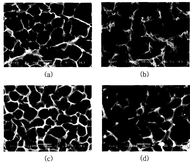
Figure 8. SEM images of freeze-dried P(NIPAAm- co -AN) hydrogels treated in water at 10 °C before drying. Feed ratio of AN (mol %); (a) 0 (PNIPAAm), (b) 4, (c) 8, and (d) 10.
