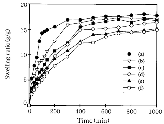
Figure 6. Swelling ratio as a function of time for P(NIPAAm-co-AN) hydrogels at 25 °C. Feed ratio of AN (mol %); (a) 0 (PNIPAAm), (b) 2, (c) 4, (d) 6, (e) 8, and (f) 10.
