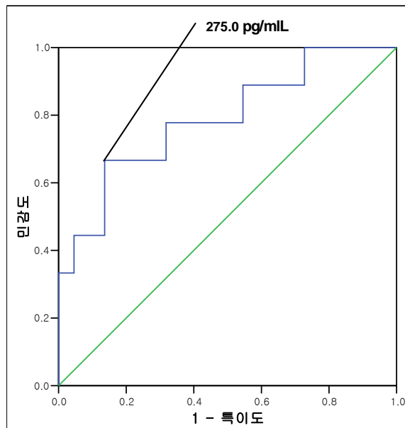
Figure 2. ROC curve.
