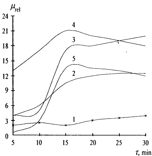
Fig. 1. Dependence of magnetic permeability on the activation time in mechano-chemical reaction processing; (1) quartz without additions, (2) quartz with additions of 5 % ethanol, (3) butanol, (4) ethylene glycol, (5) 15 % iron chloride
