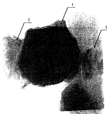
Fig. 2. Electron microscopic picture of quartz modified nano-composite particle polymerized ( \times 400,000 ), 1) polymer grafted to the particle surface, 2) polymer non-grafted (homo-polymer)
