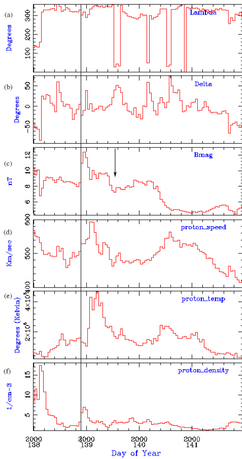
Figure 3. An IPS driven by the Ejecta on May 17, 2000 [DOY 138] The vertical solid line indicates the time of the IPS.
