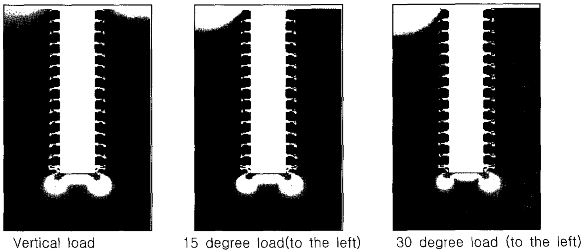
Figure 5. Stress(von Mises stress) distribution in trabecular bone with flat ended standard implant (3.0mm in diameter, 12mm in length)
