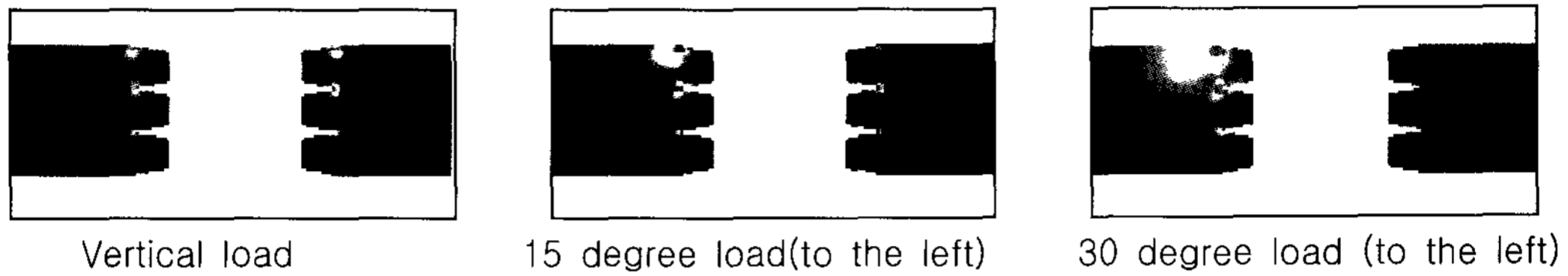
Figure 4. Stress(von Mises stress) distribution in the cortical bone with pointed ended mini implant (3.0mm in diameter, 12mm in length)
