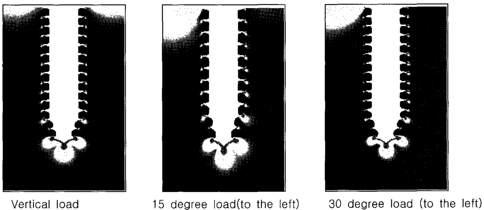
Figure 6. Stress(von Mises stress) distribution in trabecular bone with pointed ended mini implant (3.0mm in diameter, 12mm in length)
