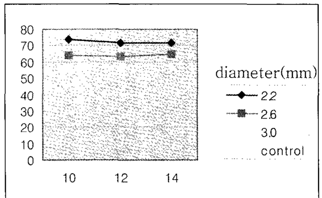
Figure 10. Maximum von Mises stress in the trabecular bone with vertically loaded mini-implant(x axis: length; mm, y axis: stress; MPa)
