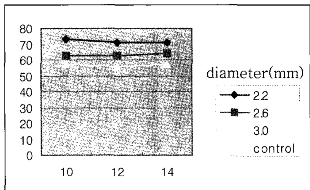
Figure 11. Maximum von Mises stress in the trabecular bone with 15 degree obliquely loaded mini-implant(x axis: length; mm, y axis: stress; MPa)
