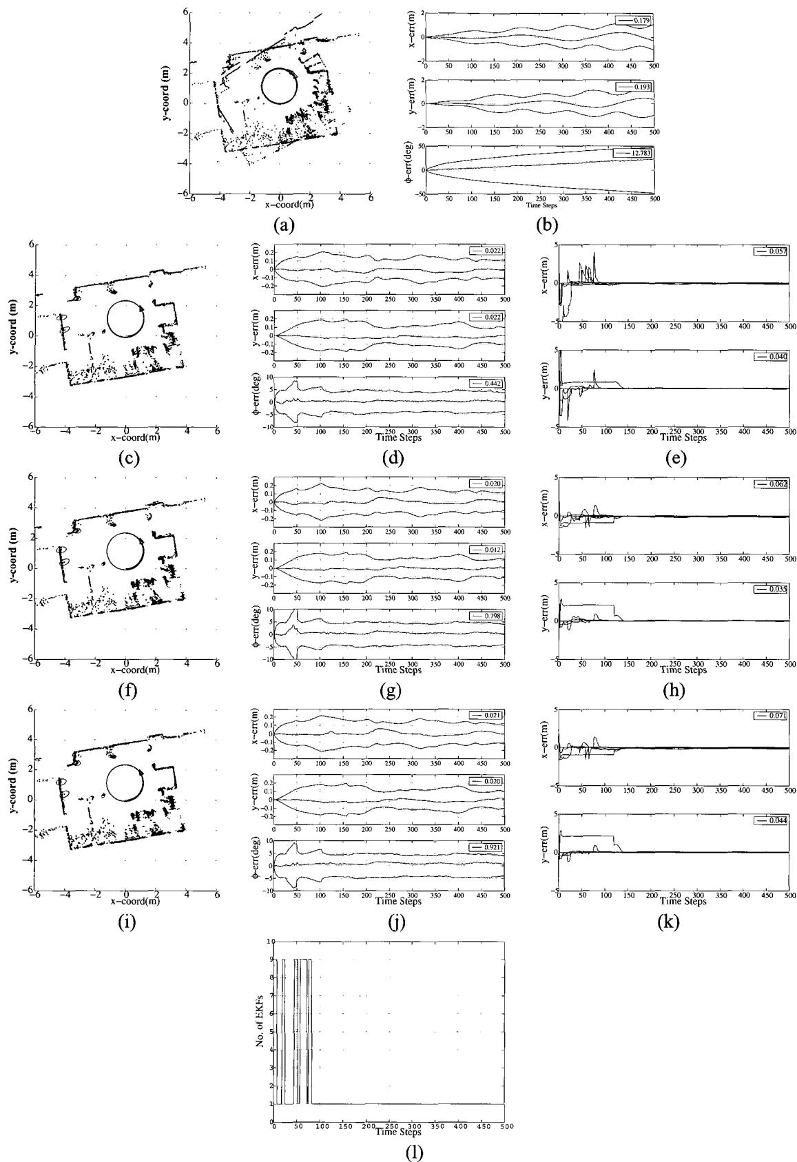
Fig. 8. SLAM results from trajectory 2: Odometer:- (a) Mapped environment; (b) Robot position error and uncertainty. EKF:- (c) Mapped environment; (d) Robot position error and uncertainties; (e) Landmark errors. Conventional GSF:- (f) Mapped environment; (g) Robot position error and uncertainties; (h) Landmark errors, Proposed GSF:- (i) Mapped environment; (j) Robot position error and uncertainties; (k) Landmark errors; (l) No. of EKFs used in the GSF.
