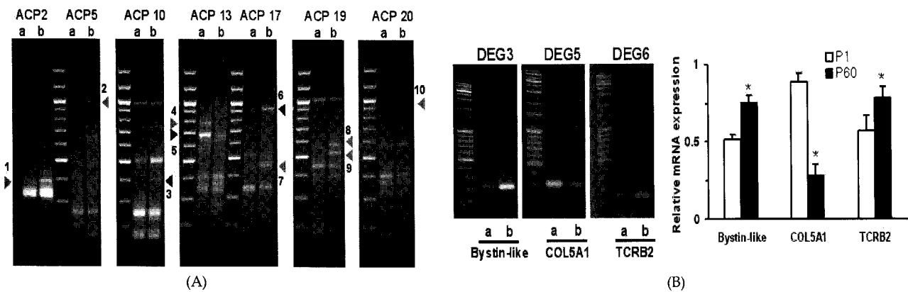
Fig. 2. Differentially expressed genes (DEGs) between neonatal and peripubertal rat thymus. (A) Gel is photographed to show DEGs obtained from thymus of different age. Using 20 ACPs, 10 DEGs were identified in P1 and P60 thymuses. Arrows indicate DEG bands (1~10). These DEG bands were excised from the gel for further cloning and sequencing. Three black triangles represent bystin-like, COL5A1, and TCRB2. ACP, annealing control primer; a, post neonatal 1 day thymus; b, post neonatal 60 days thymus. (B) Expression level of DEGs derived from P1 and P60 rat thymus using semi-quantitative RT-PCR. Data of bar graph are shown as mean±SD of triplicate determinations. COL5A1, Collagen type V alpha 1; TCRB2, T-cell receptor beta-chain segment 2.
