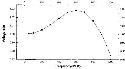
Fig. 7. Calculation results of voltage ratio.
