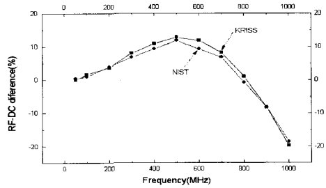
Fig. 9. Measurement results of \delta (%)
