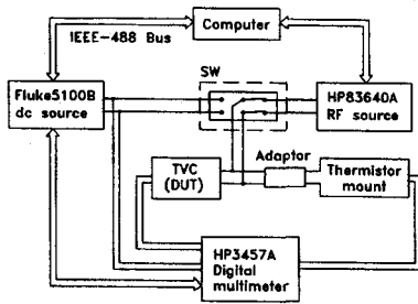
Fig. 8. Test setup.
