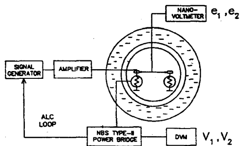
Fig. 3. Block diagram of the microcalorimeter system
