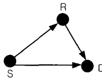
Fig. 2. Simple cooperative diversity model.
