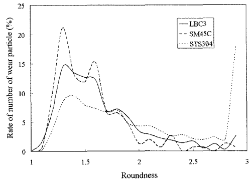
(b) Wear particles more than 4 μm
