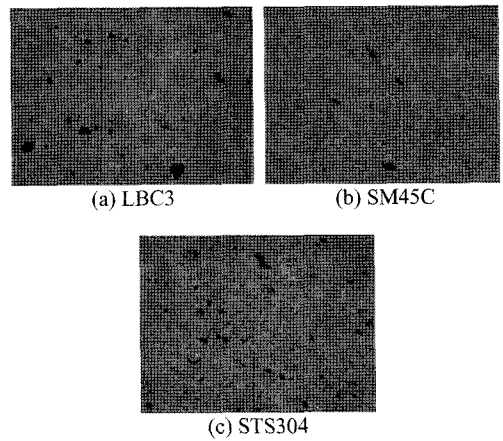
Fig. 6. Transmitted images photos. of wear particles.
