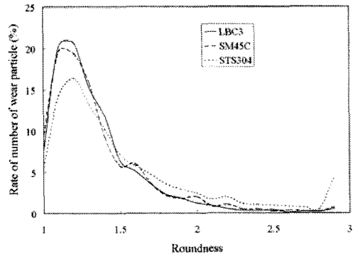
(a) Wear particles less than 4 μm
