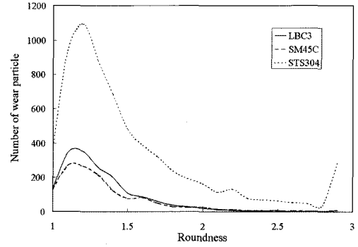
(a) Wear particles less than 4\mu\text{m}
