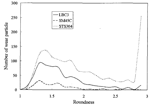
(b) Wear particles more than 4\mu\text{m}
