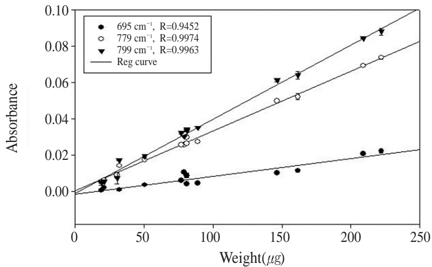
Fig. 2. Calibration curves for the quartz peaks at 695, 779 and 799 \text{cm}^{-1} .
