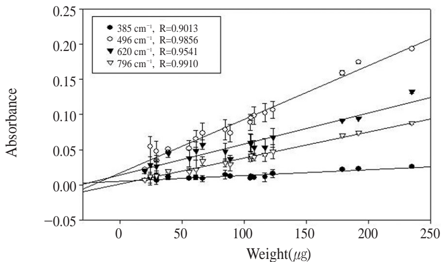
Fig. 3. Calibration curves of cristobalite
