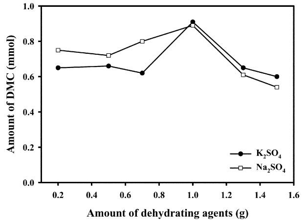
Fig. 5. Effect of the additive amount on the direct DMC synthesis over Ce 0.8 Zr 0.2 O 2 catalyst.
