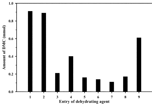
Fig. 2. Effect of the various additives on the direct DMC synthesis using MeOH and CO 2 over Ce 0.8 Zr 0.2 O 2 catalyst (1: K 2 SO 4 , 2: Na 2 SO 4 , 3: Na 2 CO 3 , 4: Li 2 CO 3 , 5: NH 4 NO 3 , 6: H 3 PO 4 , 7: P 2 O 5 , 8: Molecular sieves 3A, and 9: Only-Ce 0.8 Zr 0.2 O 2 catalyst).
