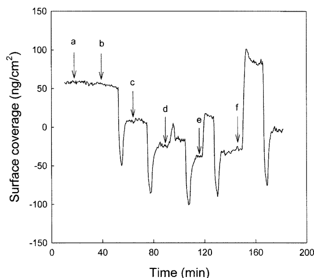
Fig. 3. Concentration-dependent responses of OWLS-based immunosensor detecting flatfish vitellogenin at anti-flatfish vitellogenin antibody dilution of 1:10 for immobilization. Five-hundred \mu l of the reaction buffer (a) and flatfish vitellogenin solutions at concentrations of 0.00675 (b), 0.0675 (c), 0.675 (d), 6.75 (e), and 67.5 nM (f) was individually injected into the system after baseline stabilization, following 10 mM HCl treatment.
