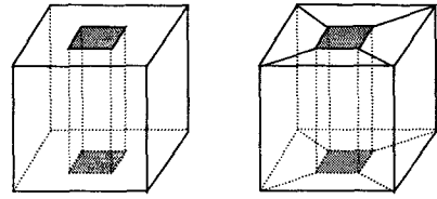
(a) v-e+f=2
