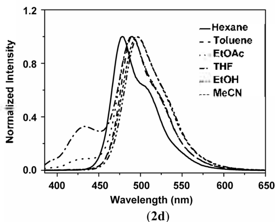
Figure 3. Normalized photoluminescence spectra of 1d and 2d in various solvents.
