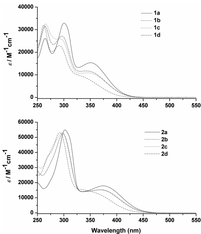
Figure 2. Absorption spectra of BP series ( 1a-1d , up) and DBP series ( 2a-2d , down) in acetonitrile ( 1.0 \times 10^{-5} M).
