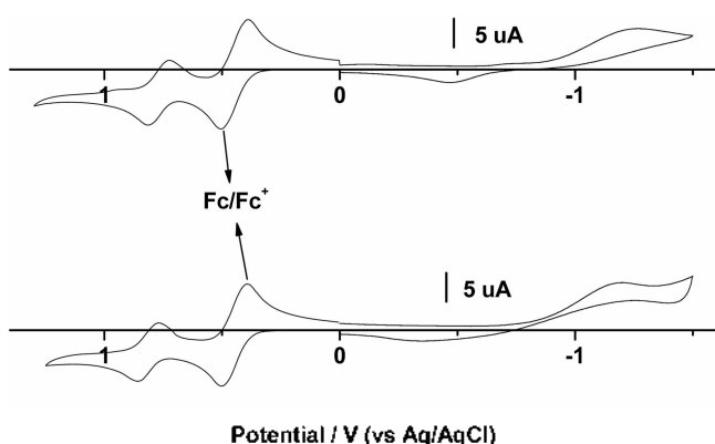
Figure 4. Cyclic voltammograms of 1 mM solutions of 1d (top) and 2d (down) in \text{CH}_2\text{Cl}_2 (oxidation process) and THF (reduction process) at a platinum electrode (0.1 M TBAPF 6 ; scan rate 100 mV/s).
