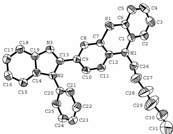
Figure 1. Crystallographic structure of 1d (ORTEP drawing).
