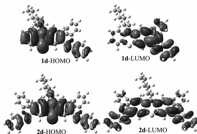
Figure 5. Pictorial presentation of HOMO (left) and LUMO (right) of 1d and 2d .
