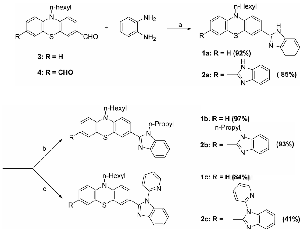
Scheme 1. Reagents and conditions: (a) \text{Na}_2\text{S}_2\text{O}_5 , DMF, 95 °C; (b) 1-bromopropane, NaI, DMF, r.t.; (c) 2-bromopyridine, CuI, 1,10-phenanthroline, \text{Cs}_2\text{CO}_3 , DMF, 110 °C.
