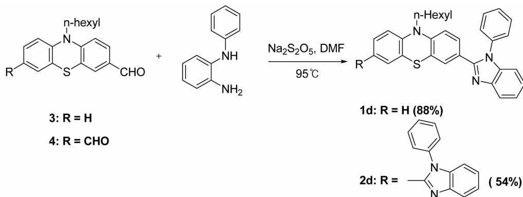
Scheme 2. The synthesis of 1d and 2d .
