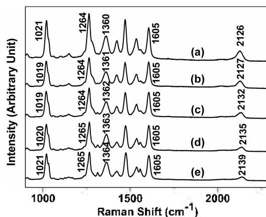
Figure 5. SERS spectra of 10^{-3} M N719 on Ag electrode at various voltages of (a) 0.8 , (b) -0.6 , (c) -0.4 , (d) -0.2 , and (e) 0.0 V vs. the standard Ag/AgCl electrode.
