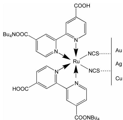
Figure 1. Molecular structure of (\text{Bu}_4\text{N})_2[\text{Ru}(\text{dcbpy})_2(\text{NCS})_2] (N719) and plausible binding on Au, Ag, and Cu metal surfaces.
