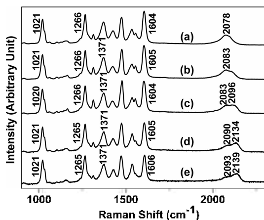
Figure 6. SERS spectra of \sim 10^{-3} M N719 on Cu electrode at various voltages of (a) -0.8 , (b) -0.6 , (c) -0.4 , (d) -0.2 , and (e) 0.0 V vs. the standard Ag/AgCl electrode.
