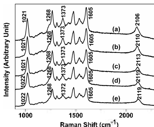
Figure 4. SERS spectra of 10^{-3} M N719 on Au electrode at various voltages of (a) -0.8 , (b) -0.6 , (c) -0.4 , (d) -0.2 , and (e) 0.0 V vs. the standard Ag/AgCl electrode.
