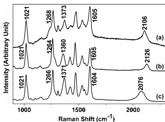
Figure 3. SERS spectra of 10^{-3} M N719 on (a) Au, (b) Ag, and (c) Cu electrode surfaces at a voltage of -0.8 V vs. the standard Ag/AgCl electrode in 900\text{--}2300\text{ cm}^{-1} . All the spectra were taken by the irradiation light source at 632.8\text{ nm} from the HeNe laser.
