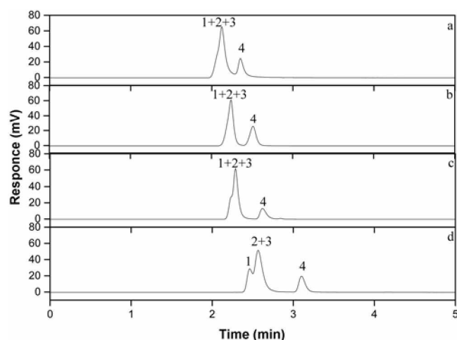
Figure 4. Chromatograms of a mixture of nucleotides with mobile phase without (a) and with 0.5 (b), 6.0 (c) and 10.0 (d) mM [EMIm][BF 4 ] (peaks numbering: (1) 5'-UMP, (2) 5'-IMP, (3) 5'-GMP, (4) 5'-TMP).
