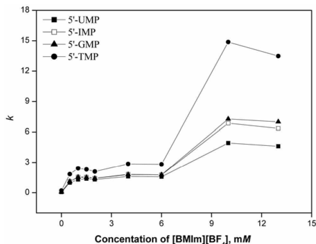
Figure 1. Retention factors ( k ) of nucleotides without and with [\text{BMIm}][\text{BF}_4] in mobile phase.
