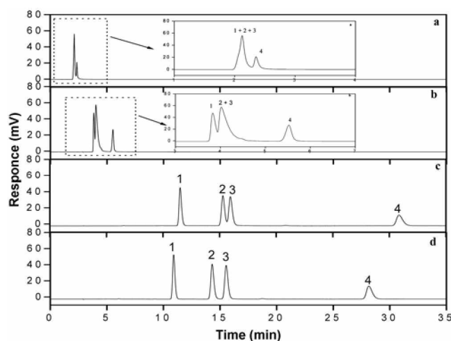
Figure 2. Chromatograms of a mixture of nucleotides with mobile phases without (a) and with 0.5 (b), 10.0 (c) and 13.0 (d) mM [\text{BMIm}][\text{BF}_4] (peaks numbering: (1) 5'-UMP, (2) 5'-IMP, (3) 5'-GMP, (4) 5'-TMP).
