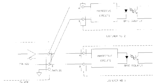
Fig. 9 Circuit diagram of NMEA-0183 protocol
