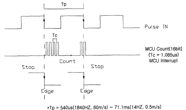
Fig. 5 Pulse signal of wind force
