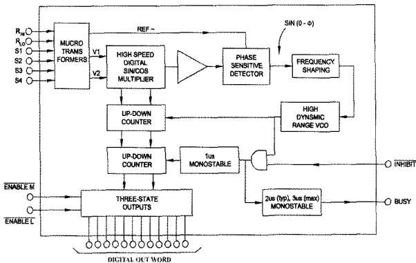
Fig. 2 Diagram of synchro signal process
