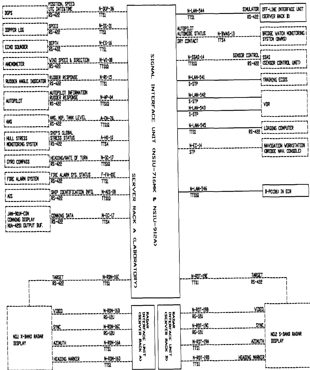
Fig. 1 An Example of Systematic diagram of ship's interface unit
