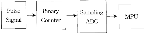
Fig. 6 Diagram of pulse signal process
