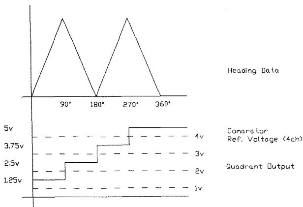
Fig. 8 Waveform of analogue H/Q signal
