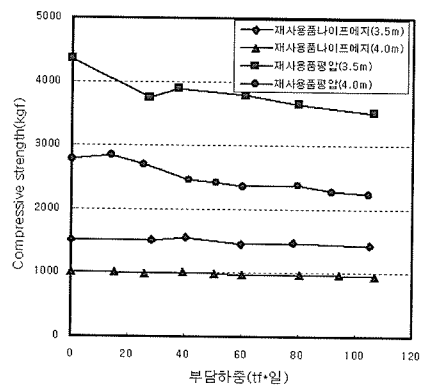
[Fig. 3] Strength change according to load carrier
