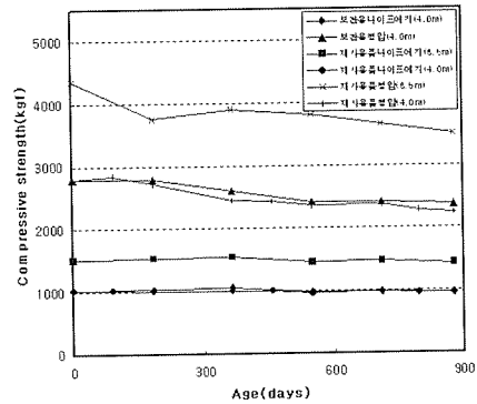
[Fig. 1] Strength change according to age
