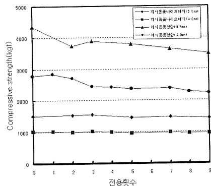
[Fig. 2] Strength change according to use frequency
