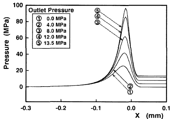
Fig. 5 Influence of outlet pressure on the pressure distribution of lubrication film (at \alpha=2.2 \times 10^{-8} \text{ m}^2/\text{N} )
