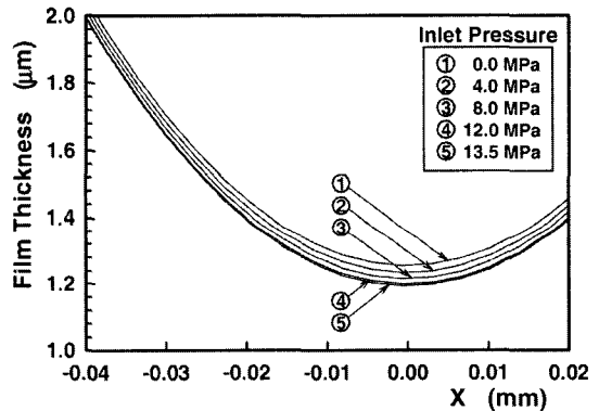
Fig. 8 Influence of inlet pressure on the film thickness (at \alpha=0 )
