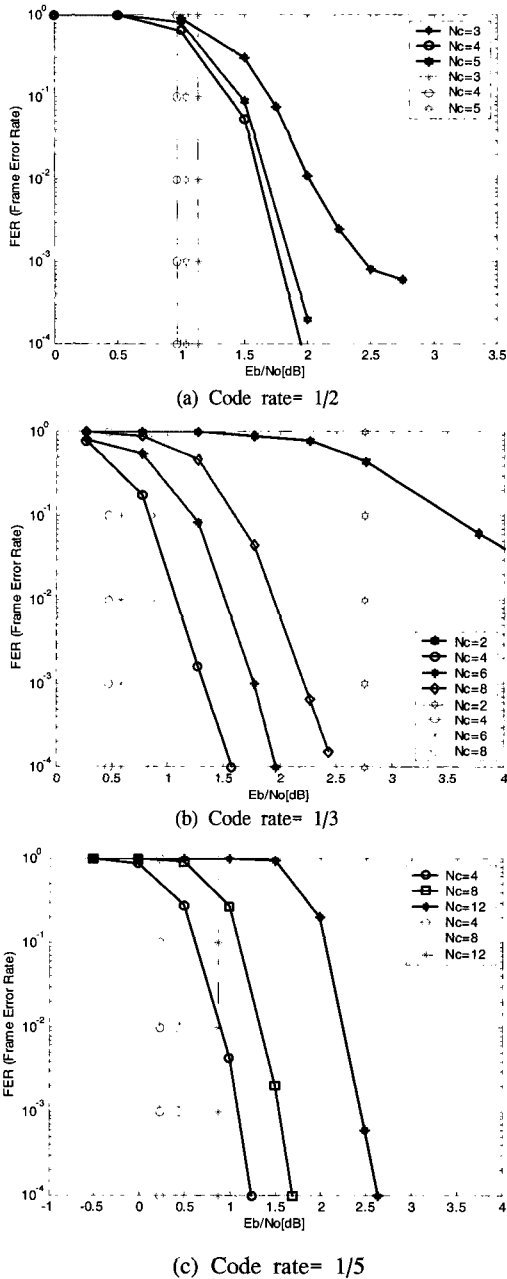
Fig.3. Comparison of various CZZ codes for a fixed rate (Dash-dot line: Threshold values, Solid line: Simulation result).
