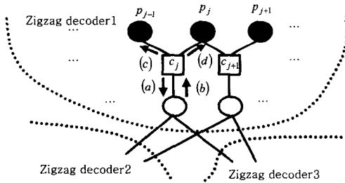
Fig.1. Message flows in CZZ decoder using two-way scheduling when Nc=3.
