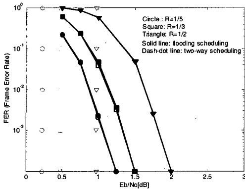
Fig.2. Comparison of CZZ codes when different schedulings are used
