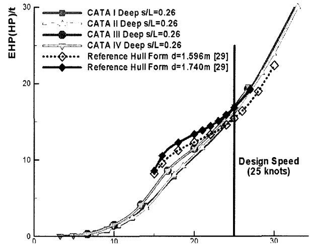
Fig. 14. Comparison of effective horse powers.
