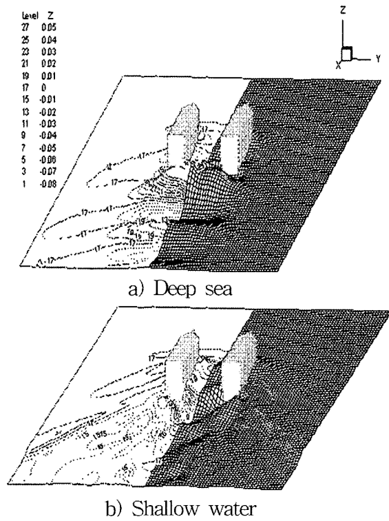
Fig. 12. Free surface contours around CATA IV at the design speed ( s/L=0.26 ).
