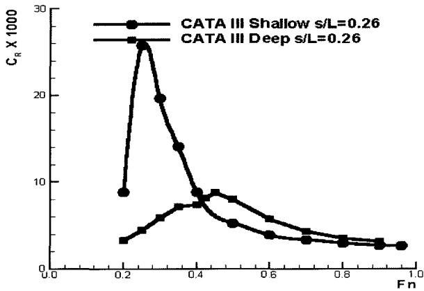
Fig. 9. Coefficients of residuary resistance CATA III in shallow and deep water conditions ( s/L=0.26 ).
