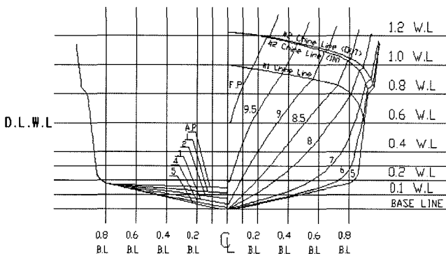
Fig. 17. Body plan of the main hull.
