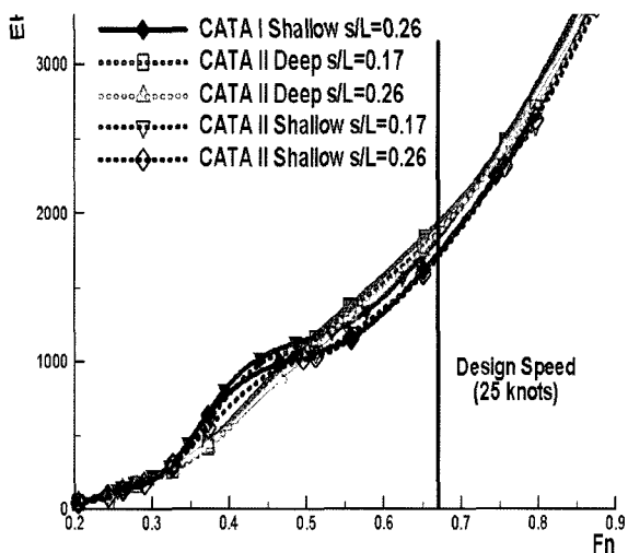
Fig. 6. EHP curves of CATA I and II.
