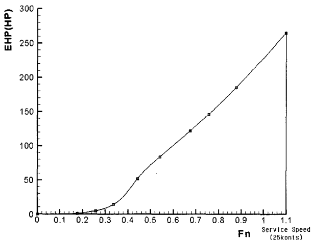
Fig. 22. EHP curve.
