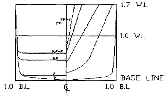
Fig. 1. The body plan of CATA I.
