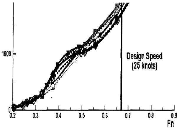
Fig. 3. EHP curves of CATA I.
