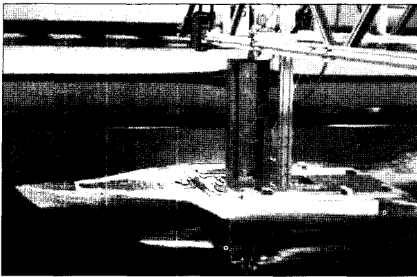
Fig. 21. Photograph of the model test (Fn=0.877).
