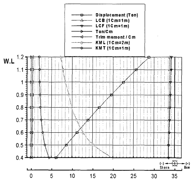
Fig. 23. Hydrostatic properties curves of trimaran.
