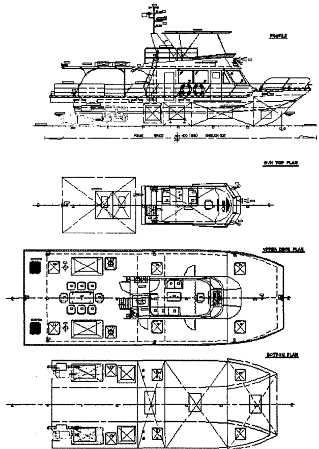
Fig. 15. General arrangements of the pleasure fishing boat.
