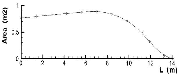
Fig. 18. Sectional area curve of the main hull.
