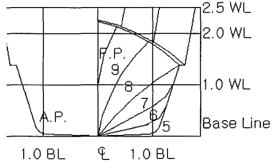
Fig. 7. The body plan of CATA III.
