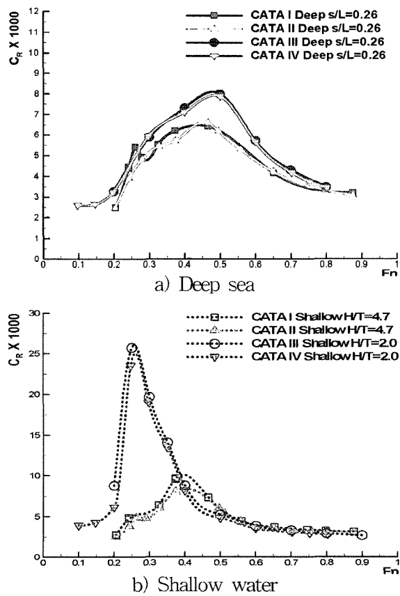
Fig. 13. Comparison of residuary resistances, C_R curves.
