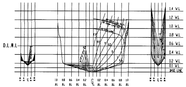
Fig. 19. Body plan of the trimaran.
