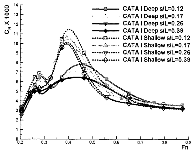
Fig. 2. Residual resistances of CATA I.
