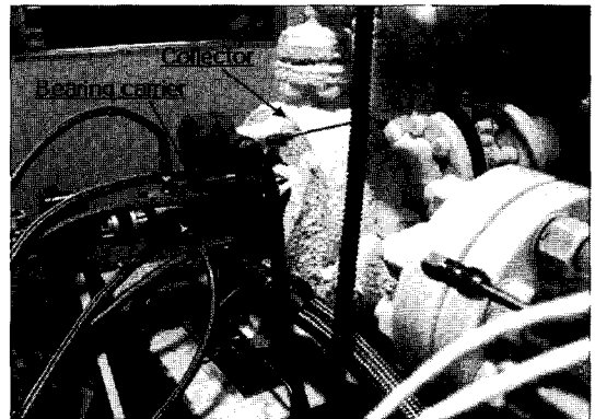
(b) Lubrication part in cryogenic environment
