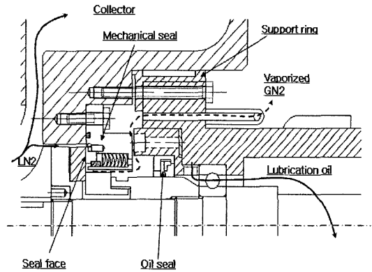
(a) View of bearing lubrication system
