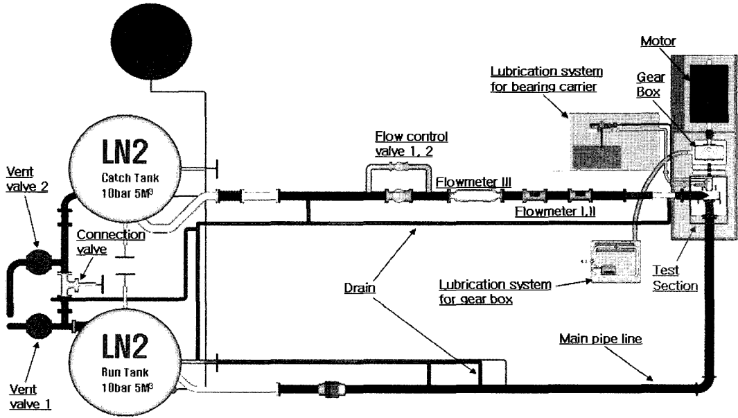
Fig. 1 Cryogenic pump test facility
