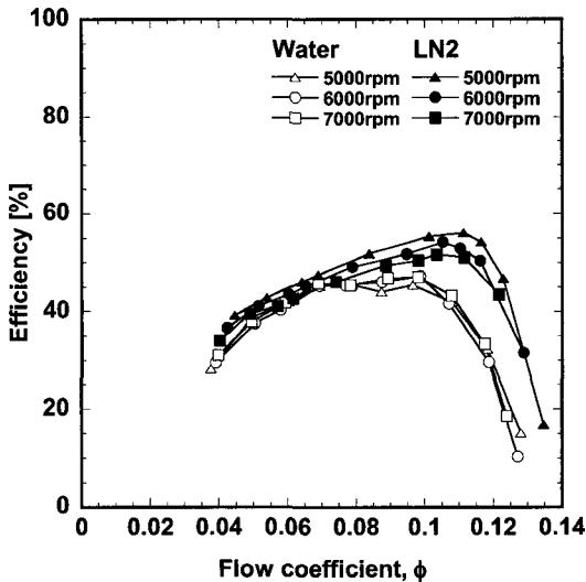
Fig. 9 Efficiency of an inducer
