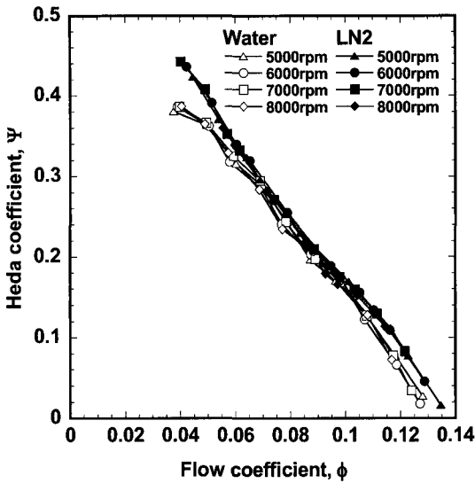
Fig. 8 Performance of an inducer
