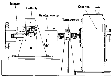
(a) Schematic of test rig
