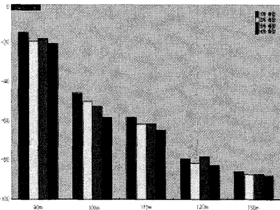
Fig. 10 S/N rate to distance in open space with secondary hedge
