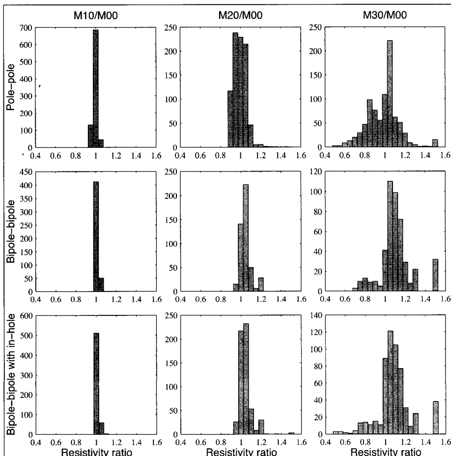
Fig. 1. Histograms of the ratio between the baseline model and the models with increasing CO 2 content. Top row: pole-pole electrode configuration (pp); middle row: bipole-bipole configuration (bb0); bottom row: bipole-bipole plus additional configurations with all electrodes in one hole (bb1).
