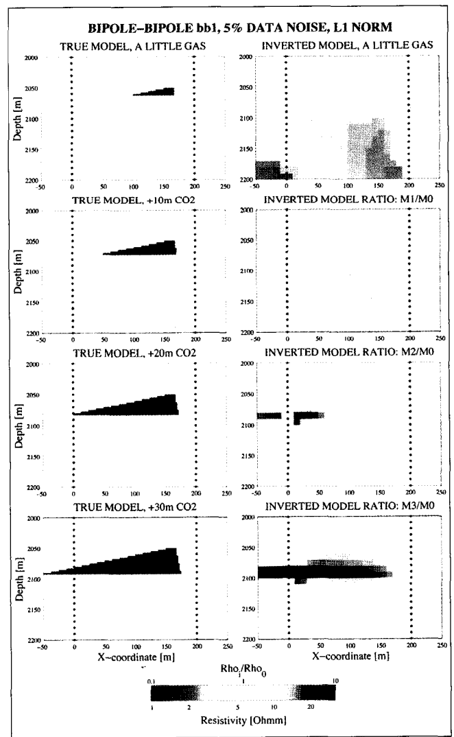
Fig. 5. In the left column is the sequence of four models illustrating an increasing CO 2 content and the borehole configurations used for ERT modelling. The right column shows the ratio between the inversion results for the bipole-bipole configurations with in-hole measurements shown in Figure 3, and the background-model result there.
