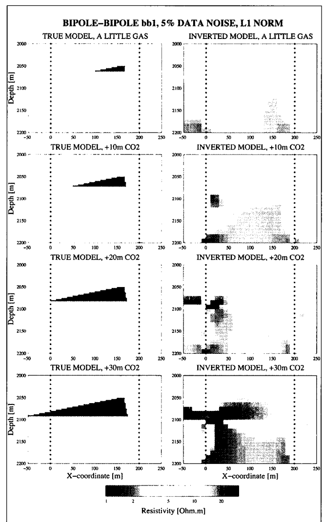
Fig. 3. In the left column is the sequence of four models illustrating an increasing CO 2 content and the borehole configurations used for ERT modelling. The right column shows the inversion results for bipole-bipole configurations with in-hole measurements, using the L1-norm.
