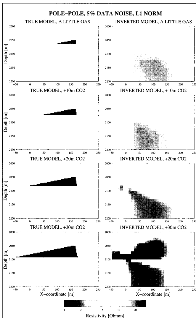
Fig. 2. In the left column is the sequence of four models illustrating an increasing CO 2 content and the borehole configurations used for ERT modelling. The right column shows the inversion results for pole-pole configurations, using the L1-norm.
