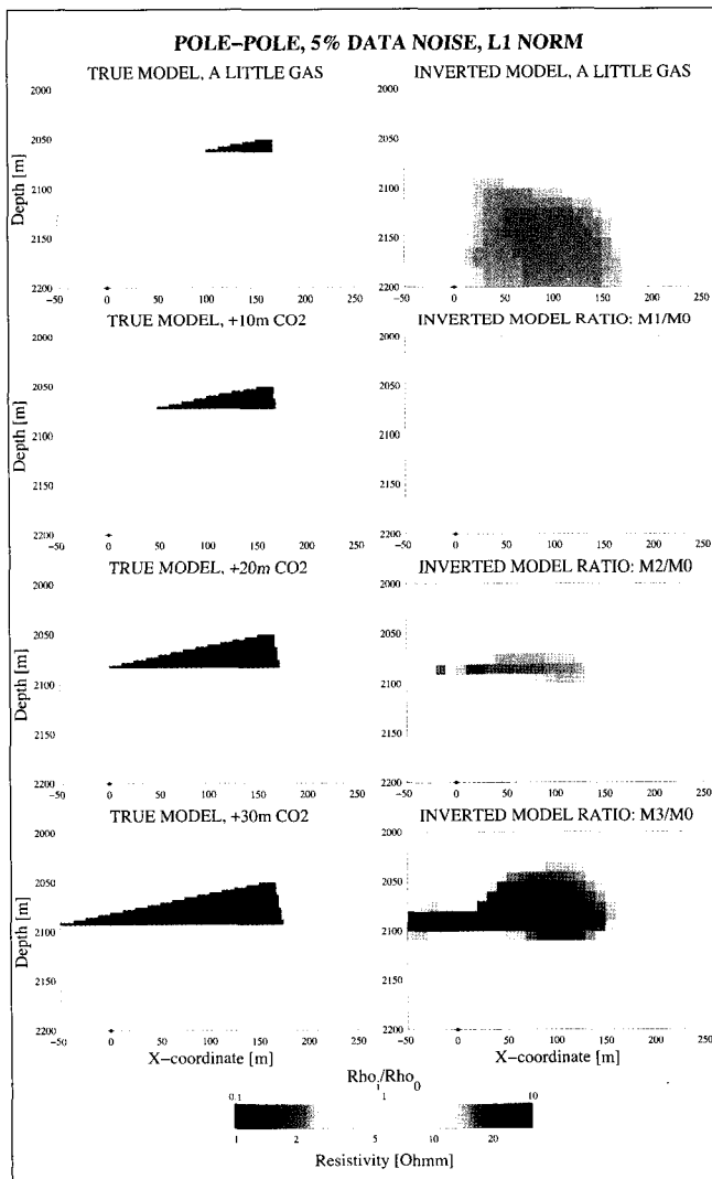
Fig. 4. In the left column is the sequence of four models illustrating an increasing CO 2 content and the borehole configurations used for ERT modelling. The right column shows the ratio between the inversion results for the pole-pole configurations shown in Figure 2, and the background-model result there.
