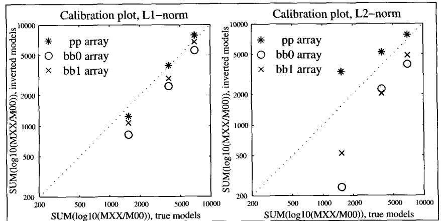
Fig. 6. The integrated resistivity change for the L1-norm and L2-norm inversions for the three electrode configurations as a function of the integrated resistivity change in the true models. The integrated resistivity change is the sum over the models of the logarithm of the change in resistivity.
