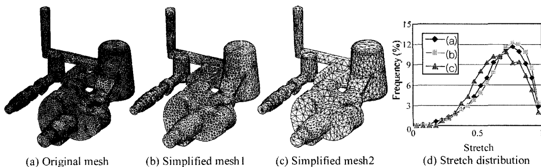
Fig. 5. Simplification results of casting part model.
