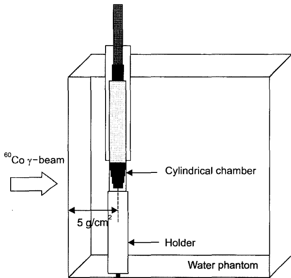
Fig. 1. The Experimental set-up for the determination of the N_{D,w} calibration factor. The absorbed doses at depth 5 \text{ g/cm}^2 in water phantom measured with a constant SSD of 100 cm and a field size of 10 \times 10 \text{ cm}^2 .
