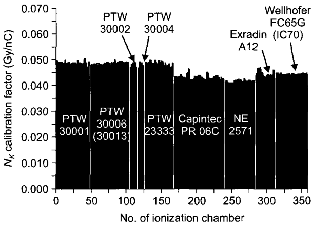
Fig. 2. The N_k calibration factor in ^{60}\text{Co} beam is a useful indicator of the uniformity within a given type a chambers. Chamber to chamber variations, demonstrated by differences in the N_k calibration factor for chambers of a given type are shown for a larger number of cylindrical chambers commonly used in radiotherapy dosimetry.
