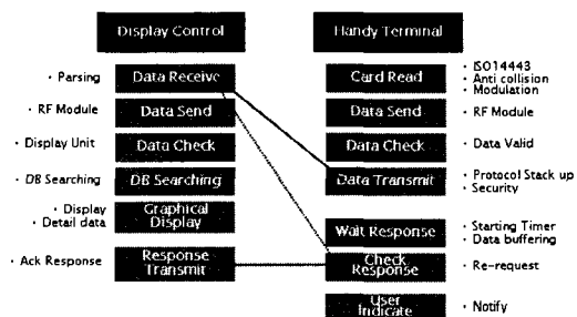
<Fig. 2> Operation Procedure
