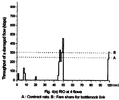
Fig. 4. TCP fairness performances of the RIO-based scheme
