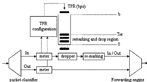
Fig. 1. The proposed ARM marker.
