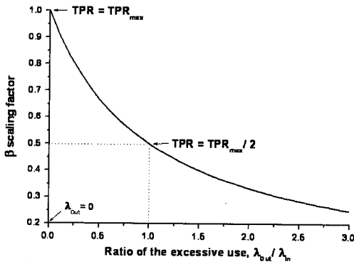
Fig. 2(b) the relation between \beta and \lambda_{out} / \lambda_{in}
