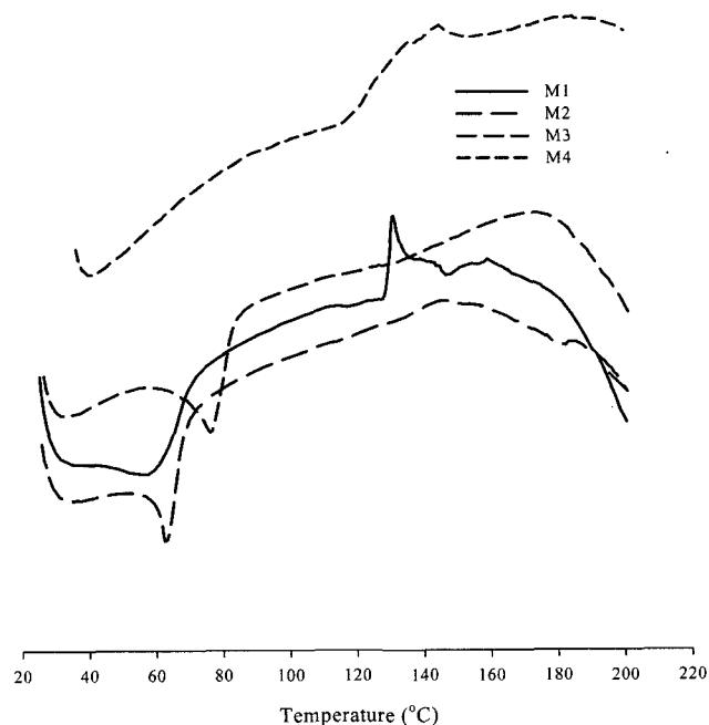
Fig. 2. DSC thermograms of the semisolid preparations with M1, M2, M3, and M4 formulations
