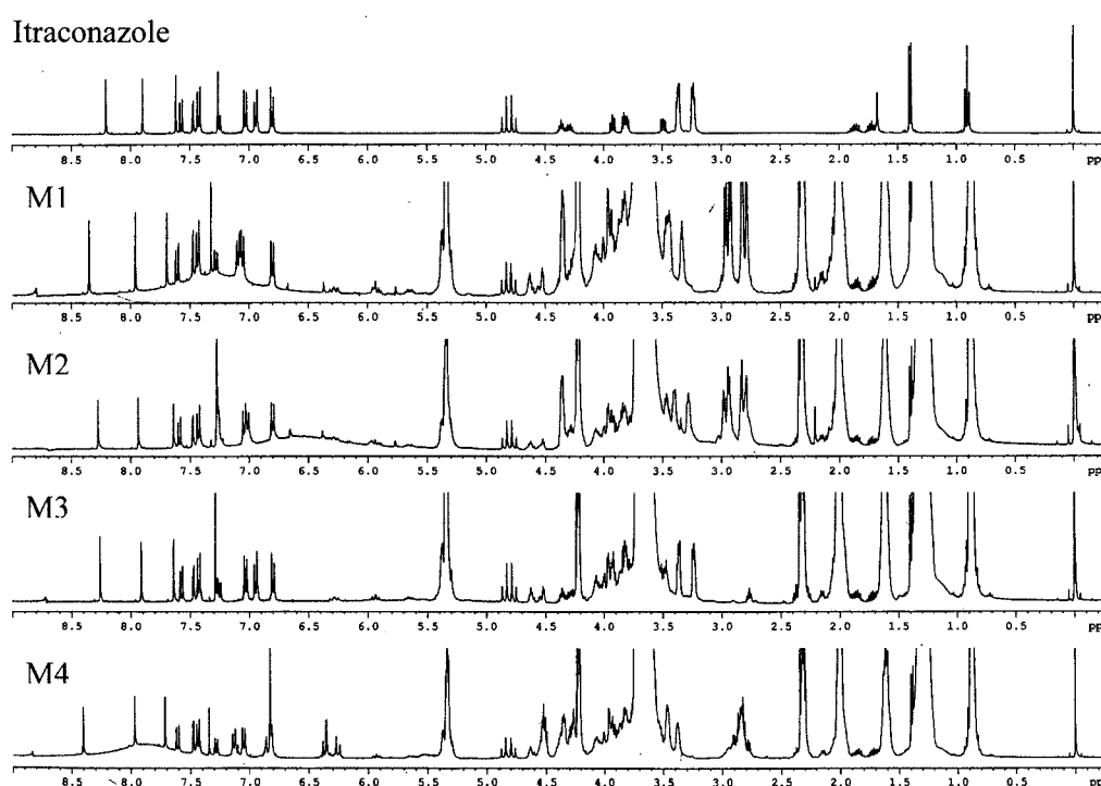
Fig. 4. 1 H-NMR spectra of itraconazole and its semisolid preparations dissolved in CDCl 3
