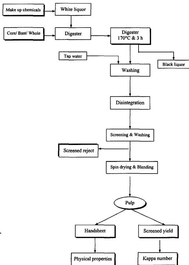
Figure 2. Flowchart of kenaf pulping by kraft process.
