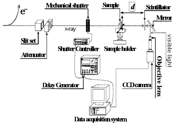
Figure 6. Schematic diagram of x-ray PIV system
