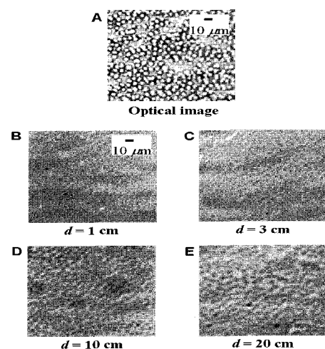
Figure 1. X-ray Images of RBC monolayer using the phase-contrast enhancement
