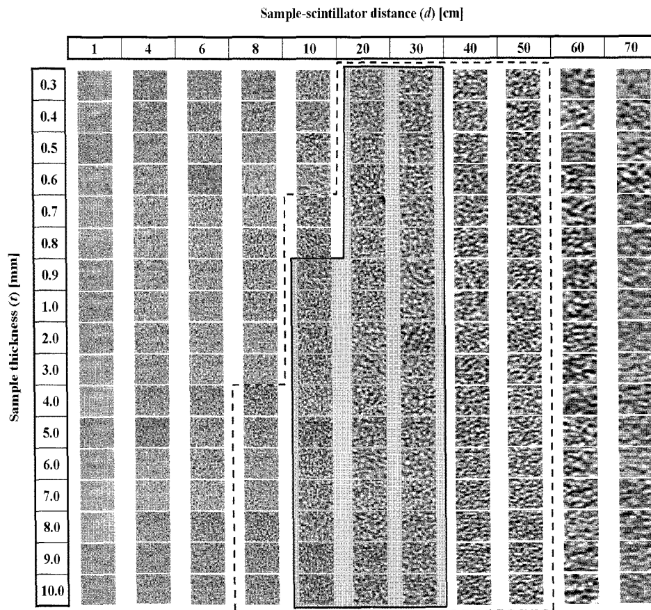
Figure 2. X-ray images of blood captured using the phase-contrast/interference-based enhancement method
