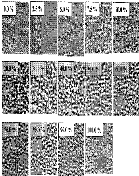
Figure 5. Speckle patterns of blood for different hematocrit( H )
