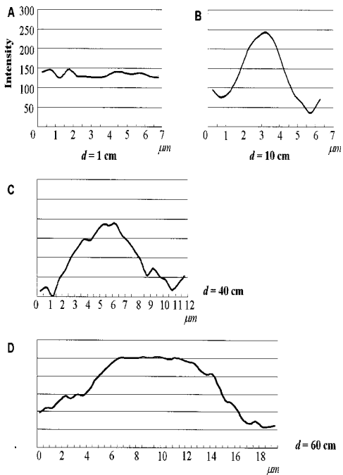
Figure 4. Intensity profiles along the horizontal direction of speckle patterns captured.
