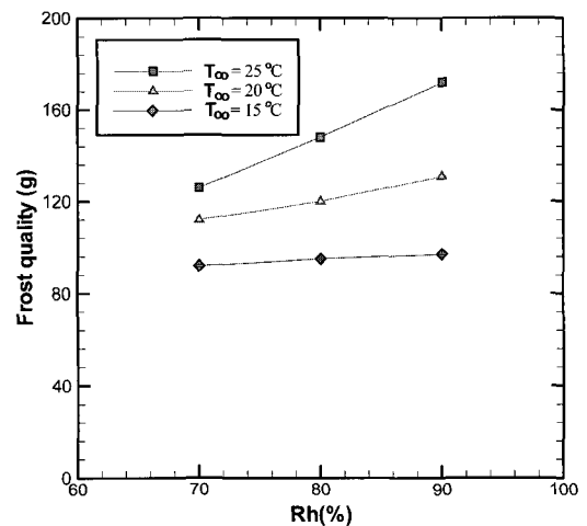
Fig. 8 Effect of relative humidity on frost quantity
