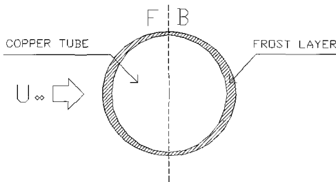
Fig. 4 Pattern of frost generation in copper tube
