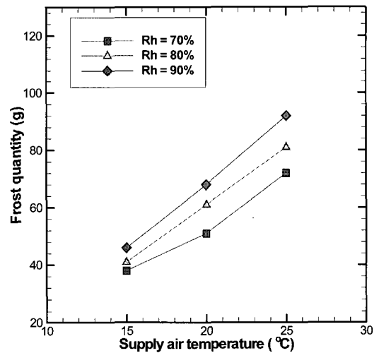
Fig. 12 Effect of supply air temperature on frost quantity
