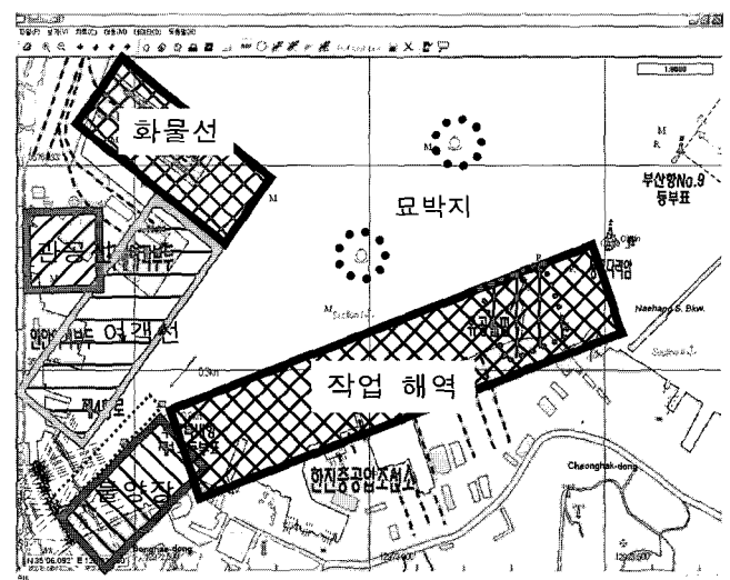
Fig. 9 functional grouping around the central wharf
