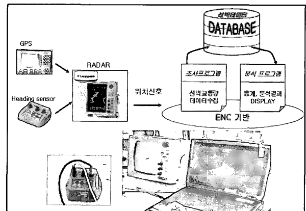
Fig. 2 Exclusive System Overview for Marine Traffic Survey
