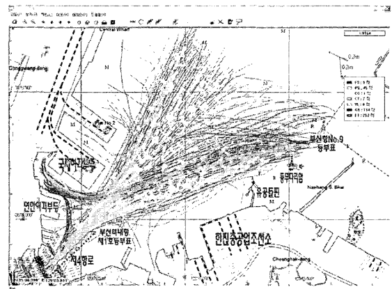
Fig. 4 Track History of No. 1 Ship Route
