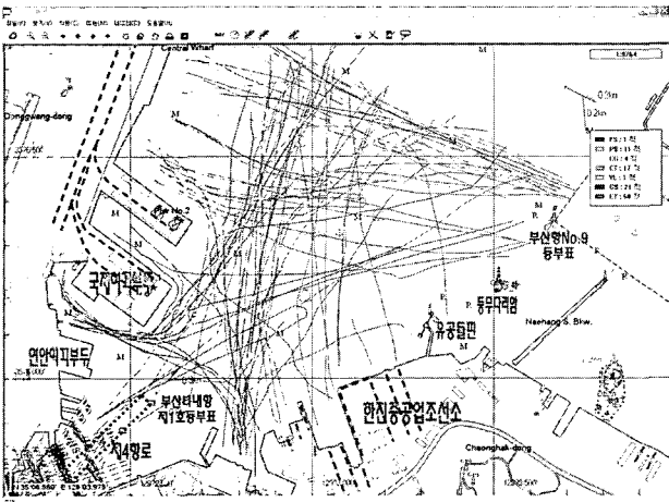
Fig. 6 Track History of No. 3, 4 and 5 Ship Route
