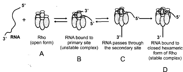
Fig. 3 Events of Rho loading and formation of ATPase competent intermediates (based on Kim and Patel 2001). RNA randomly collides with the Rho molecule forming a dynamic Rho-RNA complex. RNA then wraps around the primary binding site of each of the five protomer of the Rho open complex forming a stable moiety. The RNA subsequently passes towards the center of the open Rho ring making contact with the secondary binding site of the Rho molecule forming a steady complex. Once RNA enters the 'ring' of Rho, the open conformation gets closed by a sixth subunit, leading to the formation of a highly stable ATPase competent moiety.
