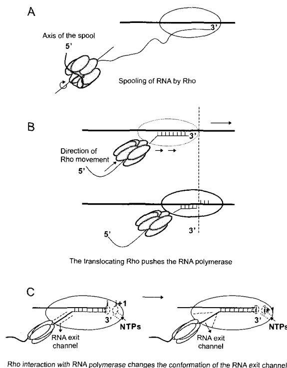
Fig. 5 Models to explain Rho's access to RNA-DNA hybrid and release RNA. A, it spools RNA from a distance without making contact with elongation complex. B, Rho forward translocates the elongation complex to get access to the RNA. C, Rho contact with elongation complex changes the conformation of RNA exit channel.
