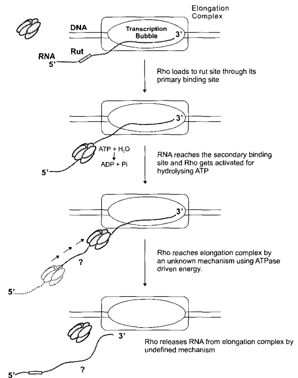
Fig. 2 An overview of the steps involved in the termination by Rho. The exact phenomenon of Rho translocation, interaction with elongation complex and finally unwinding and releasing RNA are still ambiguous.
