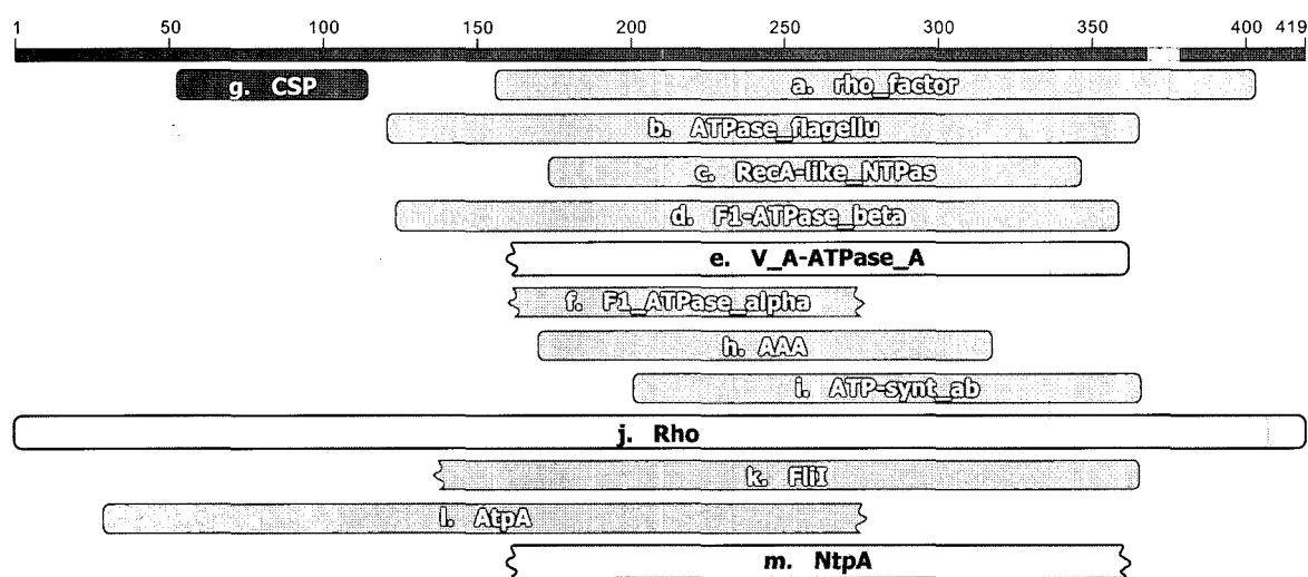
Fig. 6 Schematic representation of the conserved domains of E. coli Rho through NCBI Blast. a. Rho-factor: Transcription termination factor Rho is a bacterial ATP-dependent RNA/DNA helicase. b. ATPase-flagellum or Flagellum-specific ATPase/type III secretory pathway virulence-related protein: This group of ATPases are responsible for the export of flagellum and virulence-related proteins. The bacterial flagellar motor is similar to the F_0F_1 -ATPase, in that they both are proton driven rotary molecular devices. c. RecA-like NTPases: This family includes the NTP binding domain of F1 and V1 H^+ ATPases, DnaB and related helicases as well as bacterial RecA and related eukaryotic and archaeal recombinases. d. F_1 ATP synthase beta subunit, nucleotide-binding domain: The F-ATPase is found in bacterial plasma membranes, mitochondrial inner membranes and in chloroplast thylakoid membranes. It uses a proton gradient to drive ATP synthesis and hydrolyzes ATP to build the proton gradient. e. V/A-type ATP synthase catalytic subunit A. These ATPases couple ATP hydrolysis to the build up of a H^+ gradient, but V-type ATPases do not catalyze the reverse reaction. The Vacuolar (V-type) ATPase is found in the membranes of vacuoles, the golgi apparatus and in other coated vesicles in eukaryotes. f. F_1 ATP synthase alpha, central domain. The F-ATPase is found in bacterial plasma membranes, mitochondrial inner membranes and in chloroplast thylakoid membranes. g. CSP, Cold shock protein domain; RNA-binding domain that functions as a RNA-chaperone in bacteria and is involved in regulating translation in eukaryotes. Contains sub-family of RNA-binding domains in the Rho transcription termination factor. h. AAA-ATPases associated with a variety of cellular activities. i. ATP synthase alpha/beta family, nucleotide-binding domain. This family includes the ATP synthase alpha and beta subunits the ATP synthase associated with flagella. j. Rho: Transcription termination factor. k. Flagellar biosynthesis/type III secretory pathway ATPase: involved in cell motility and secretion / Intracellular trafficking and secretion. l. AtpA: F_0F_1 -type ATP synthase, alpha subunit involved in energy production and conversion. m. NtpA: Archaeal/vacuolar-type H^+ -ATPase subunit A involved in energy production and conversion.
