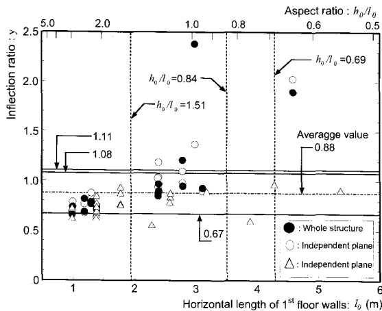
<Fig 4> Relationship between inflection height ratio and horizontal length of masonry walls
