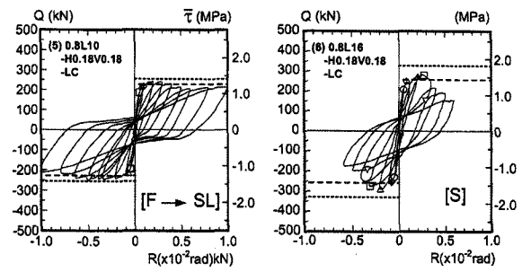
<Fig. 8> Q - R hysteresis loops of H0.18V0.18-18-LC series
