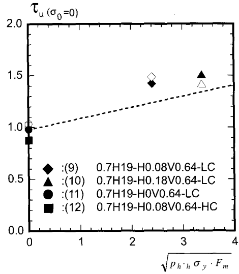
〈Fig. 11〉 \tau_{u(\sigma_0=0)} and \sqrt{P_h \cdot h \sigma_y \cdot F_m} relations
