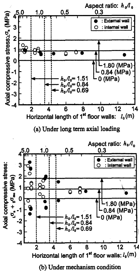
<Fig. 3> Relationship between axial compression and horizontal length of masonry walls
