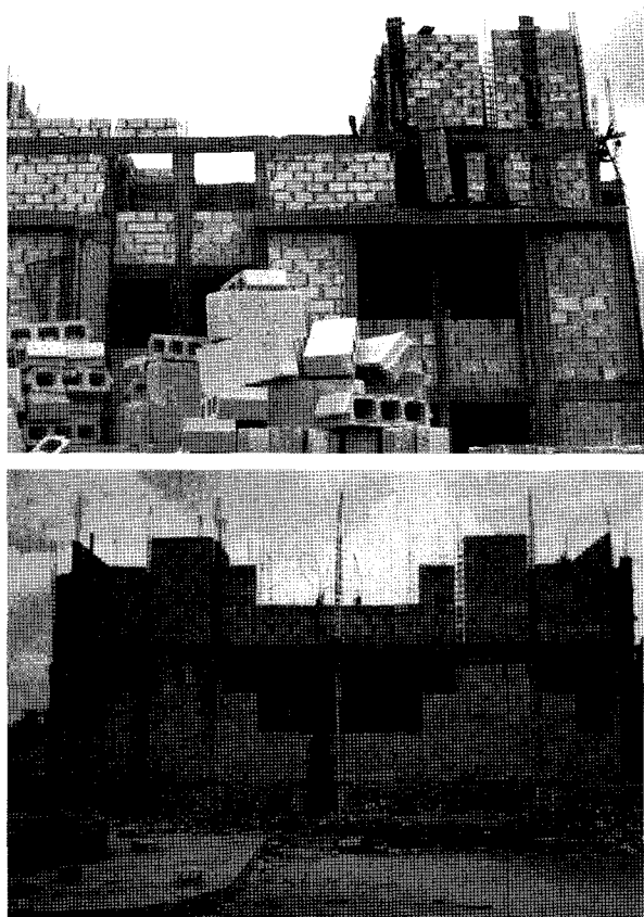
<Fig. 1> CM wall buildings under construction (Mexico, 1993)
