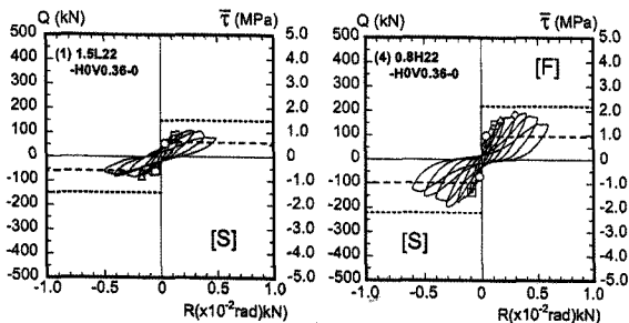
<Fig. 7> Q - R hysteresis loops of H0V0.36-0 series
