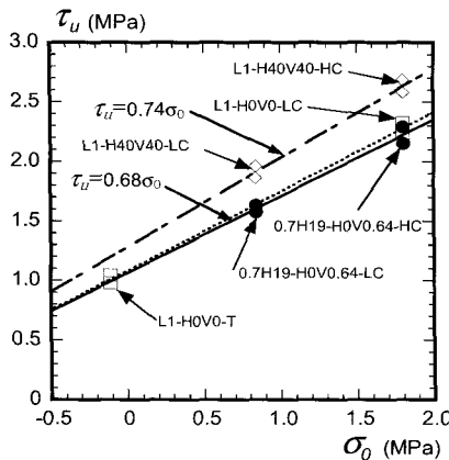
〈Fig. 10〉 Ultimate shear stress( t_u ) and vertical axial stress( \sigma_0 )
