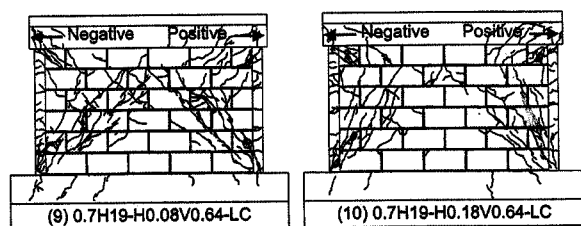
(c) Specimens with aspect ratio( h_0/l_0 ) of 0.69
