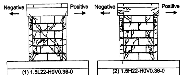
(a) Specimens with aspect ratio( h_0/l_0 ) of 1.51
