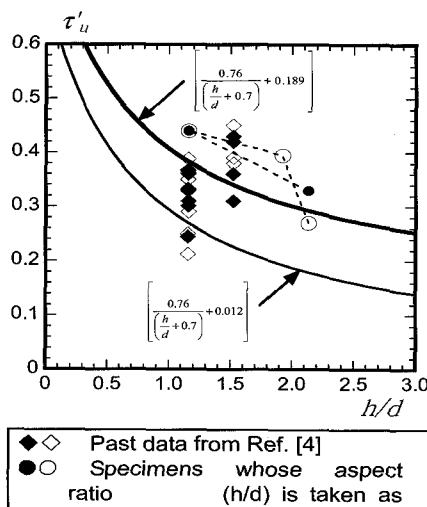
<Fig. 12> Aspect ratio ( h/d ) shear stress ( \tau'_u ) relationship
