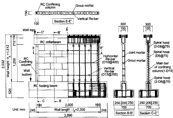
<Fig 2> Typical test specimen
