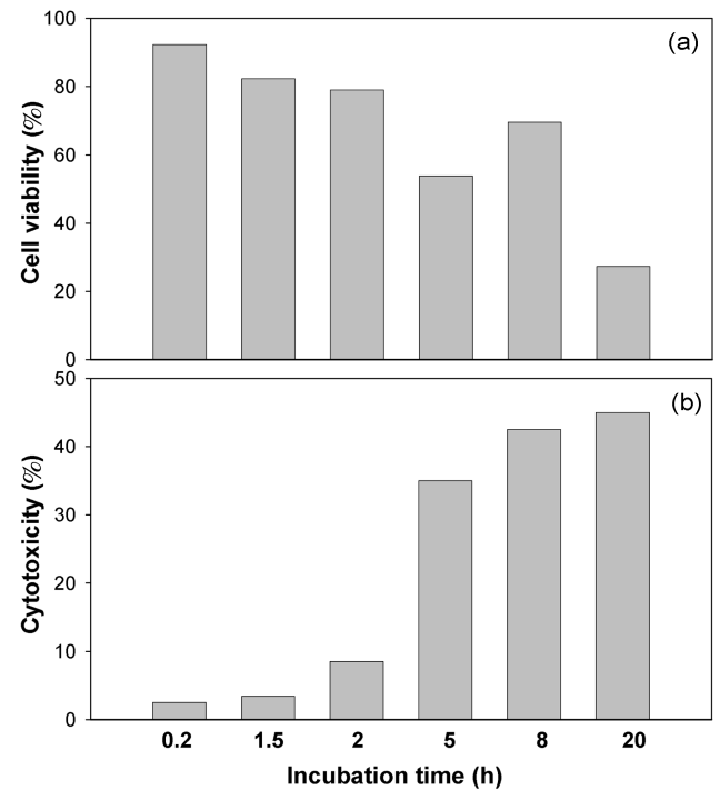
Fig. 5. Effects of incubation time with 10X concentrated vMT-GFP baculovirus on (a) cell viability and (b) cytotoxicity. MOI was 30, initial cell number was 9 \times 10^6 cells ml^{-1} , post-infection was 24 h, and post-induction was 42 h.
