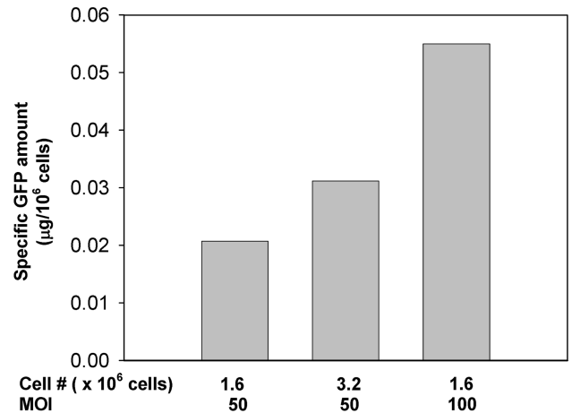
Fig. 2. Effects of MOI and initial cell number on GFP production in vMT-GFP baculovirus/S2 cells. Incubation time was 1.5 h, post-infection time was 24 h, and post-induction time was 42 h. Comparison of specific GFP expression for 60 mm dish culture.
